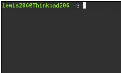
bash-Shell
